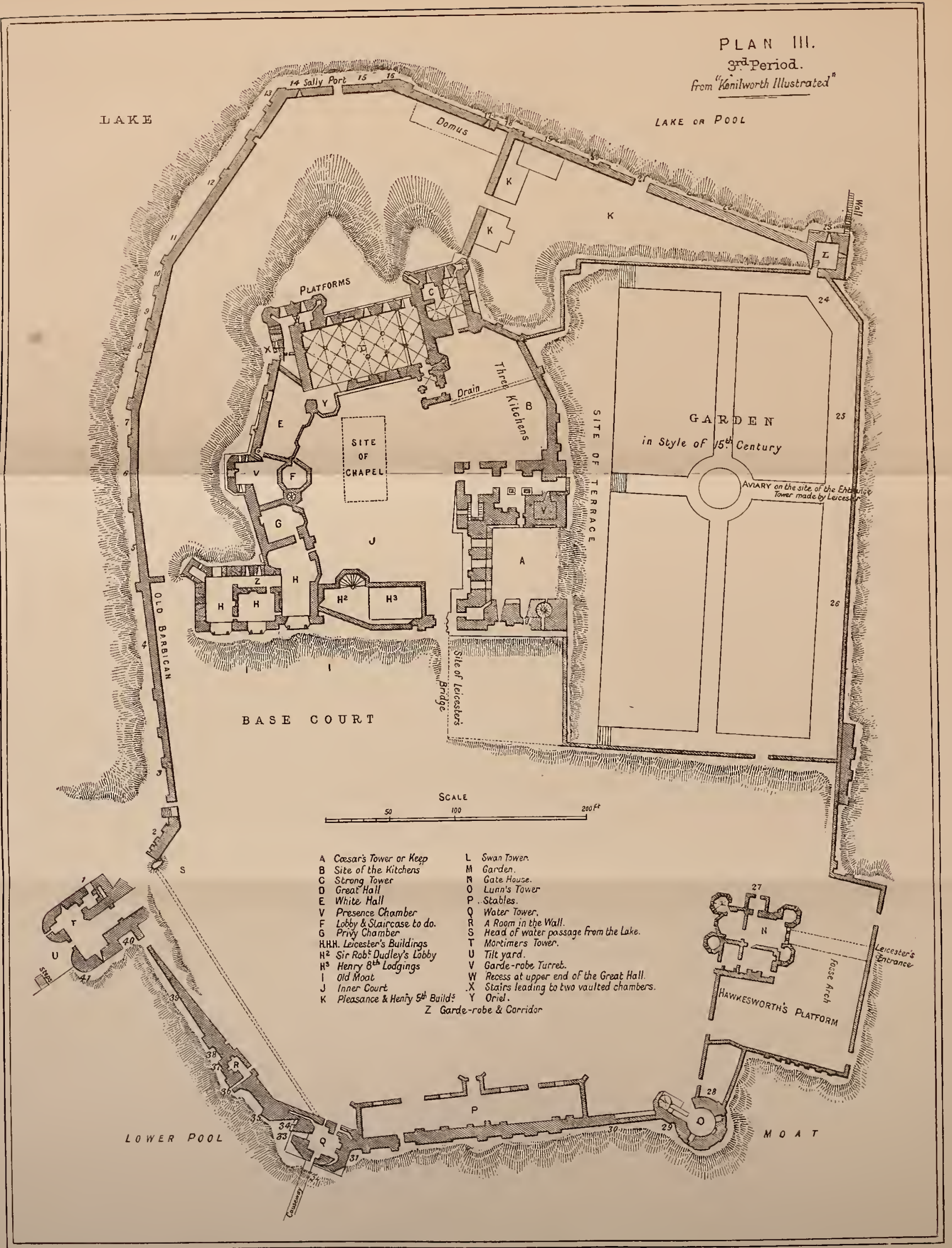
GROUND PLAN OF KENILWORTH CASTLE.
